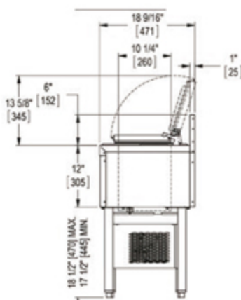
End view ice cream cabinet
