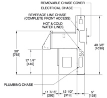
PEDESTAL BASE END VIEW
