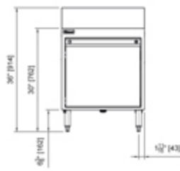
Front view storage bin
