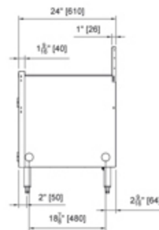
End view storage cabinet
