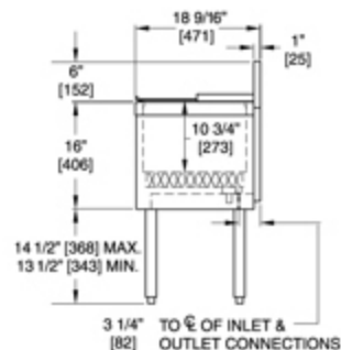
End View Standard Ice Chest
