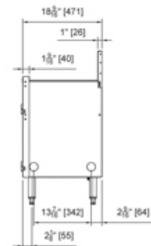
End view storage cabinet with sink
