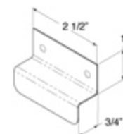
57420 (Millwork panel clip)
