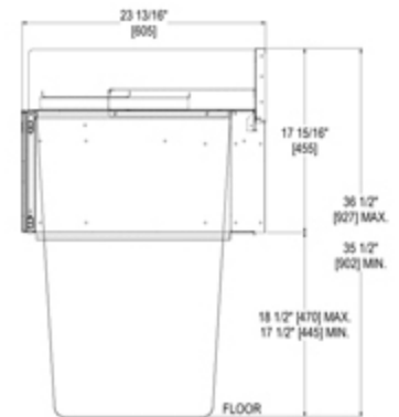
End view trash receptacle
